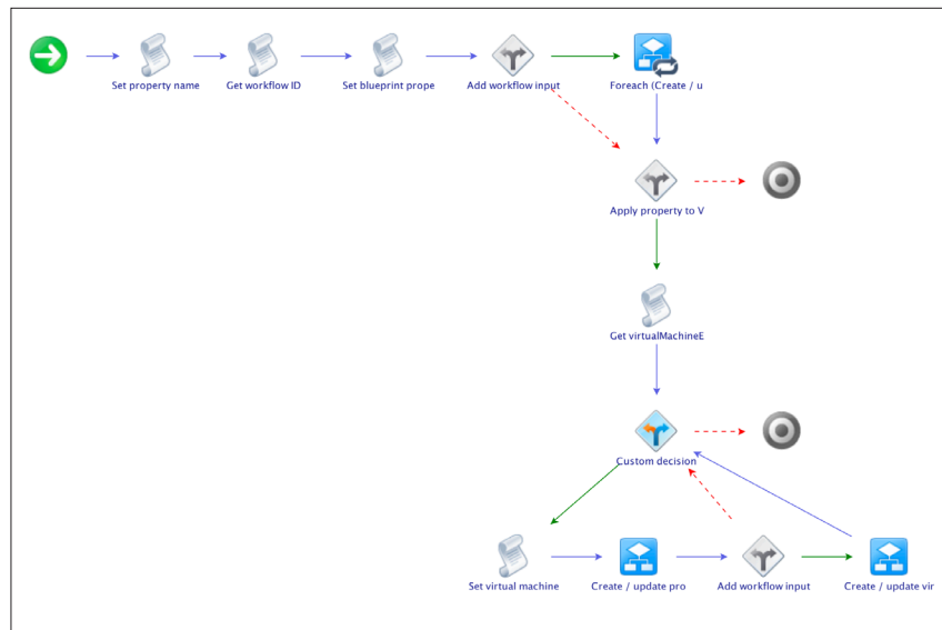
Figure 1: vRealize Orchestrator workflow visualizer
