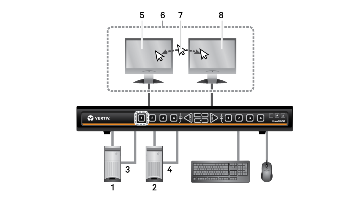
Figure 2.18 Dual-head KVM Preset
