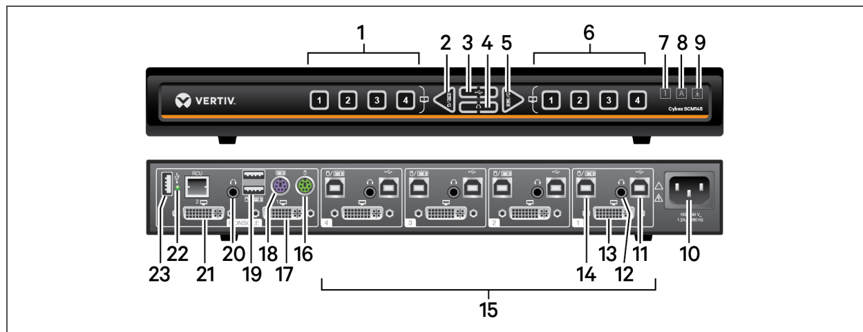
Figure 2.1 Cybex SCM 145 Secure Desktop Matrix Switch
