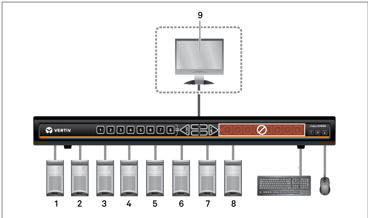
Figure 2.17 Legacy Mode Configuration
